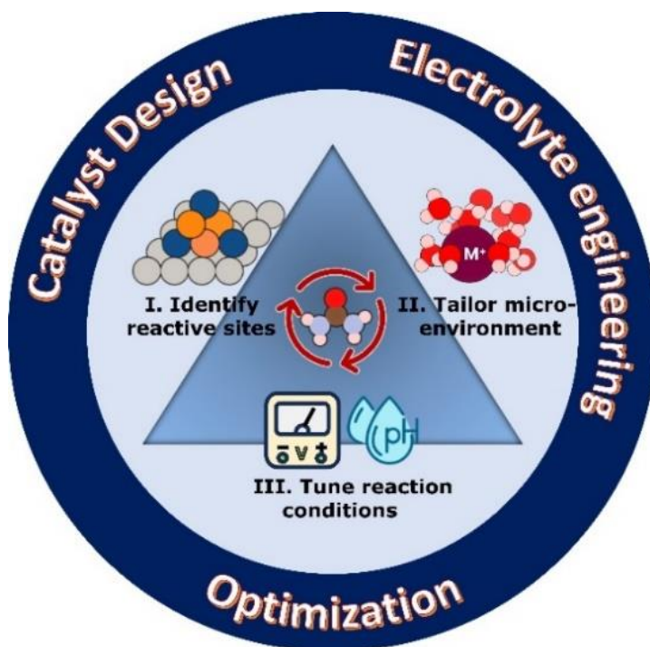
Figure 1. The proposed workflow for sustainable urea synthesis involves: i) development of reactive bimetallic catalysts, ii) electrolyte composition engineering to enhance adsorption of reaction intermediates, and iii) optimization of reaction conditions to maximize the selectivity of the designed electrocatalysts.
